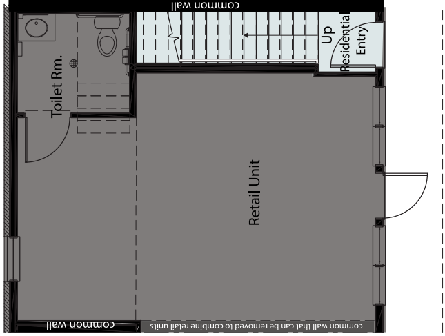
1st FLOOR - 12ft ceilings
