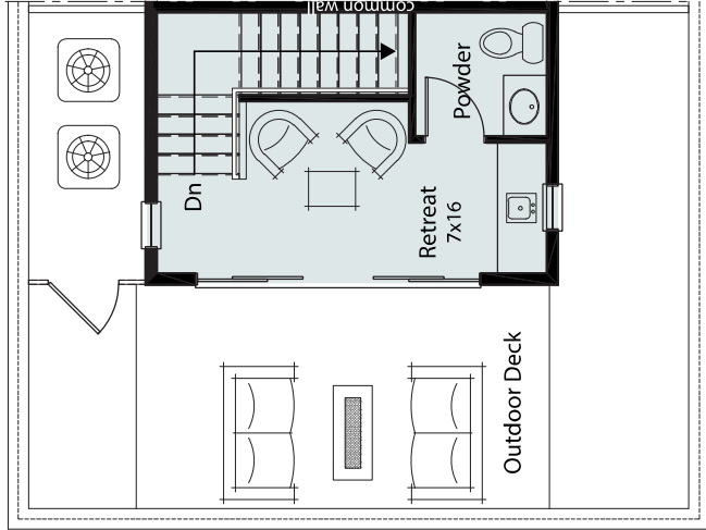
Penthouse - 9ft ceilings
