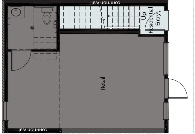
1st FLOOR - 12ft ceilings
